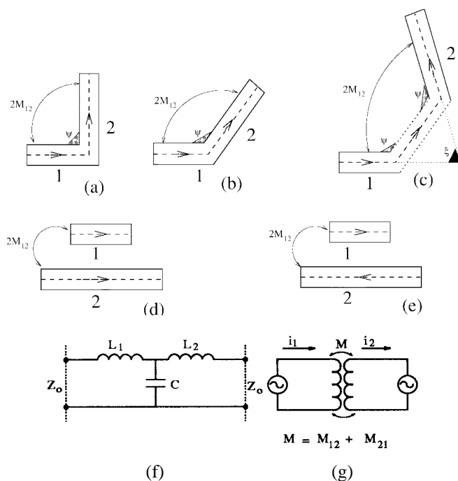
Fig. 1. Segment pair combinations contributing to any spiral configuration and their common equivalent circuit. The arrows indicate the current direction and \theta is the segment resolution.
